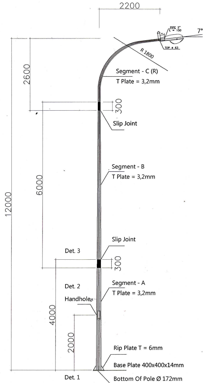
TIANG PJU H-12M SINGLE PARABOLE SCALE 1 : 25 OCTAGONAL
