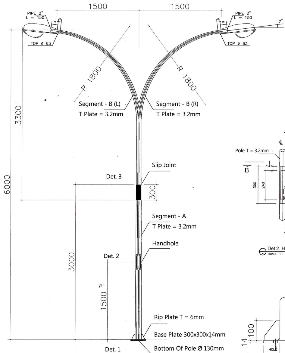
TIANG PJU H-06M DOUBLE PARABOLE SCALE 1 : 25 OCTAGONAL
