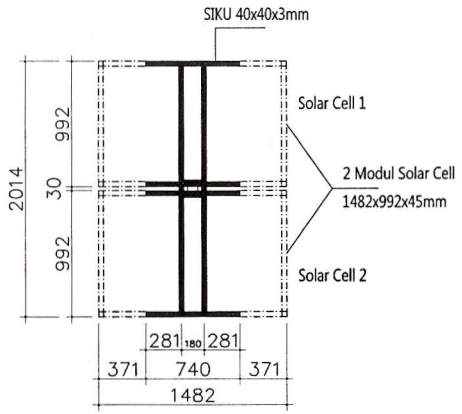
Det 5. Bracket Modul Solar Cell SCALE 1 : 25
