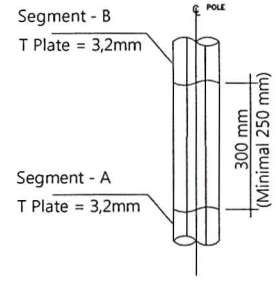
Det 3. Slip Joint SCALE 1 : 25
