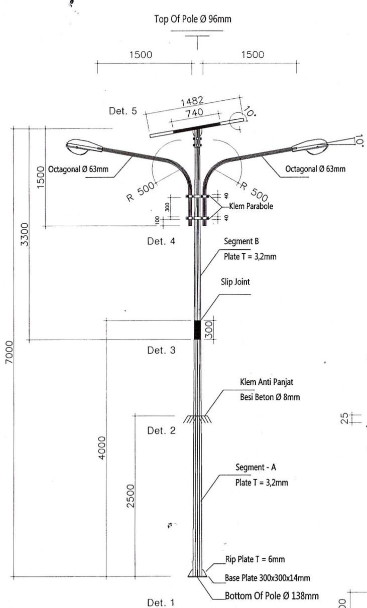
TIANG PJU H-07M DP TYPE SC SCALE 1 : 100 OCTAGONAL
