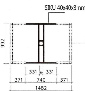
Det 3. Bracket Modul Solar Cell SCALE 1 : 25
