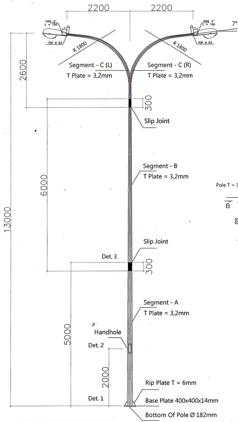
TIANG PJU H-13M DOUBLE PARABOLE SCALE 1 : 25 Octagonal
