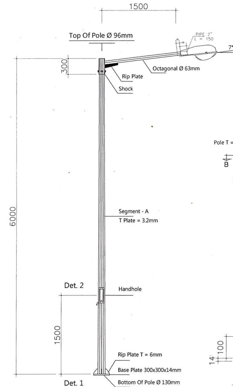
Tiang PJU H-06 M Single T SCALE 1 : 25 OCTAGONAL
