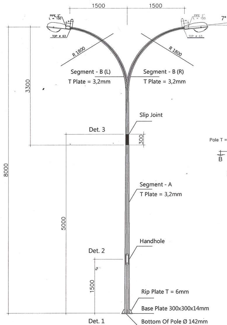
TIANG PJU H-08M DOUBLE PARABOLE OCTAGONAL SCALE 1 : 25
