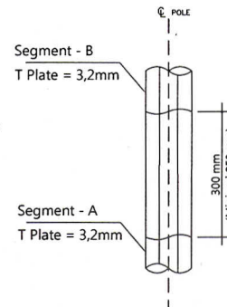
Det 3. Slip Joint SCALE 1 : 25
